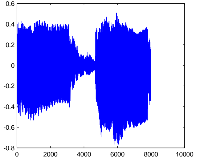
Fig. 2. First reference synchronization symbol captured from Tmote Invent speaker
