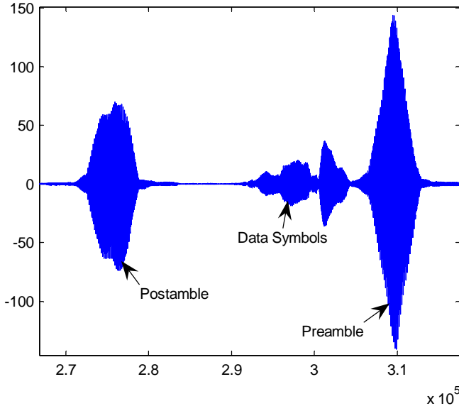
Fig. 3. Correlation output with the first reference signal
